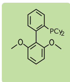
Sphos*
